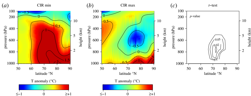
Figure 7. Composites of the latitudinal profile of air temperature anomalies (compared with 1981–2010) at 90°E to 90°W from the NCEP reanalysis for the 2007/8 CIR period and smoothed, for (a) CIR minima and (b) CIR maxima. (c) shows the probability ( p -value) from a t -test (using the unsmoothed data), that the difference arises from chance. (Online version in colour.)
