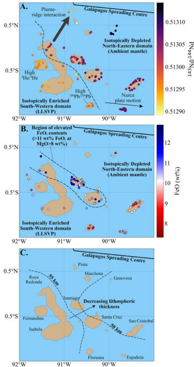
Figure 2. Variation in the composition of basalts erupted across the Galapagos Archipelago. (a) Spatial variations in the ^{143}\text{Nd}/^{144}\text{Nd} composition of the Galapagos basalts. Less radiogenic, and thus more enriched, Nd isotope signatures are observed in the south-western Galapagos. The enriched isotopic signature of Pinta is likely related to the transfer of compositionally enriched melts to the nearby Galapagos Spreading Centre (Gleeson & Gibson, 2021). (b) Variations in the \text{FeO}_t content of high-MgO basalts erupted in the Galapagos (basalts with MgO contents above 8 wt% are shown). Notably, areas with the highest \text{FeO}_t contents are found in the north and central Galapagos, on the islands of Santiago, Santa Cruz, Roca Redonda, and on the northern margins of Isabela. (c) Contours of lithospheric thickness (taken from Gibson and Geist [2010]) reveal the lithosphere thins eastwards in the Galapagos Archipelago. Data from Allan and Simkin (2000), Bow and Geist (1992), Geist et al. (2002, 2005, 2006), Gibson et al. (2012), Gibson and Geist (2010), Harpp et al. (2003), Harpp and Weis (2020), Kurz and Geist (1999), McBirney and Williams (1969), Naumann et al. (2002), Saal et al. (2007), Standish et al. (1998), Swanson et al. (1974), Teasdale et al. (2005), and White et al. (1993).
