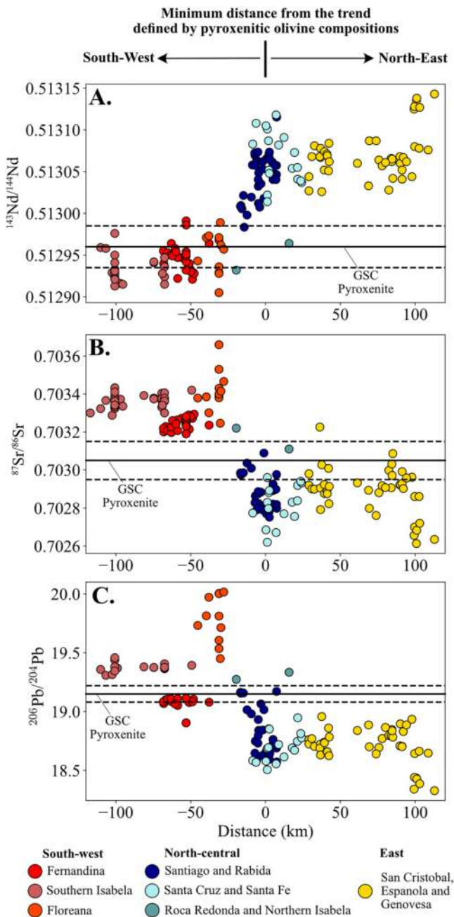
Figure 5. Radiogenic isotope composition of basalts from the Galápagos Archipelago. In all panels, the proposed isotopic composition of the pyroxenitic component identified in the source region of the Galápagos Spreading Center basalts is shown by the black horizontal lines. These values are taken from the work of Gleeson, Gibson, and Williams (2020), and Gleeson and Gibson (2021) and the uncertainties in these isotopic compositions were constrained using the python code presented in Gleeson and Gibson (2021). Basalts from Roca Redonda, northern Isabela, and the most enriched basalts from Santiago, have very similar isotopic systematics to this proposed end-member. Data from Allan and Simkin (2000), Bow and Geist (1992), Geist et al. (2002, 2005, 2006), Gibson et al. (2012), Gibson and Geist (2010), Harpp et al. (2003), Harpp and Weis (2020), Kurz and Geist (1999), McBirney and Williams (1969), Naumann et al. (2002), Saal et al. (2007), Standish et al. (1998), Swanson et al. (1974), Teasdale et al. (2005), and White et al. (1993).
