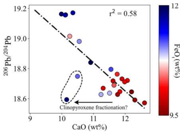
Figure 7. Correlation between the major element systematics of the high-MgO Santiago basalts (MgO >8 wt%) and radiogenic isotopes. Strong correlations that are significant at the 95% confidence level are observed between CaO or FeO i and the radiogenic isotope ratios considered in this study (e.g., 206 Pb/ 204 Pb) and confirm the relationship between isotopic enrichment and pyroxenitic contribution in the central Galápagos. Two samples with low CaO contents and unradiogenic 206 Pb/ 204 Pb signatures might result from unfiltered clinopyroxene fractionation, but we expect the influence of plagioclase and clinopyroxene fractionation to be minor in most Galápagos basalts considered here (see Supporting Information S1). Data from Gibson et al. (2012).
