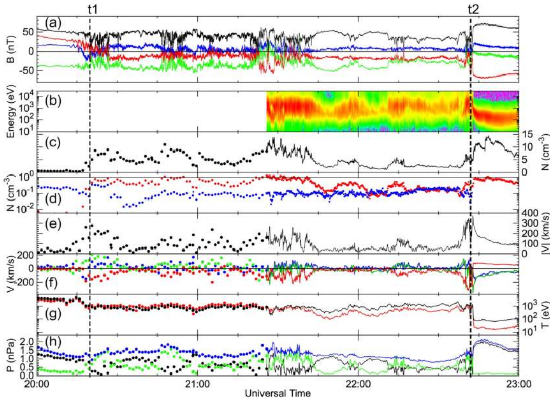
Figure 4. Outbound magnetopause crossing into the Anomalous Reconnection Layer, at the time labeled t1, and subsequent transition into the magnetosheath, at time t2. Format is the same as in Figure 3. No O + densities are shown in panel (d) after 22:40 UT because of “bleed over” from the high H + flux. Note that Fast Plasma Investigation plasma data are not available until about 21:20 UT.
