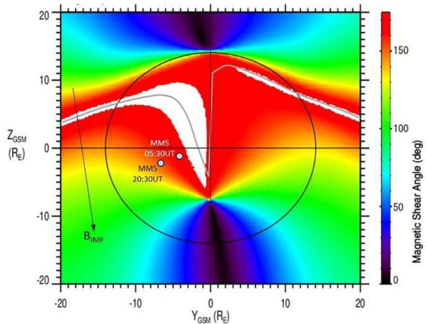
Figure 10. The magnetic shear angle across the dayside magnetopause averaged over the interval from 20:30 to 05:30 UT, with the shear angle coded as shown by the color bar on the right. The view is from the Sun and the shear is projected onto the GSM ( Y, Z )-plane, and so is the location of Magnetospheric Multiscale spacecraft at the beginning and end of the time interval. The black arrow labeled B_{IMF} shows the interplanetary magnetic field (IMF) direction averaged over the time interval. The average tilt of the Earth's dipole was -28^\circ . The thin black circular line is the terminator. White regions mark the positions where field lines are antiparallel to within 3^\circ , and the thin gray line is for precisely 180^\circ shear.
